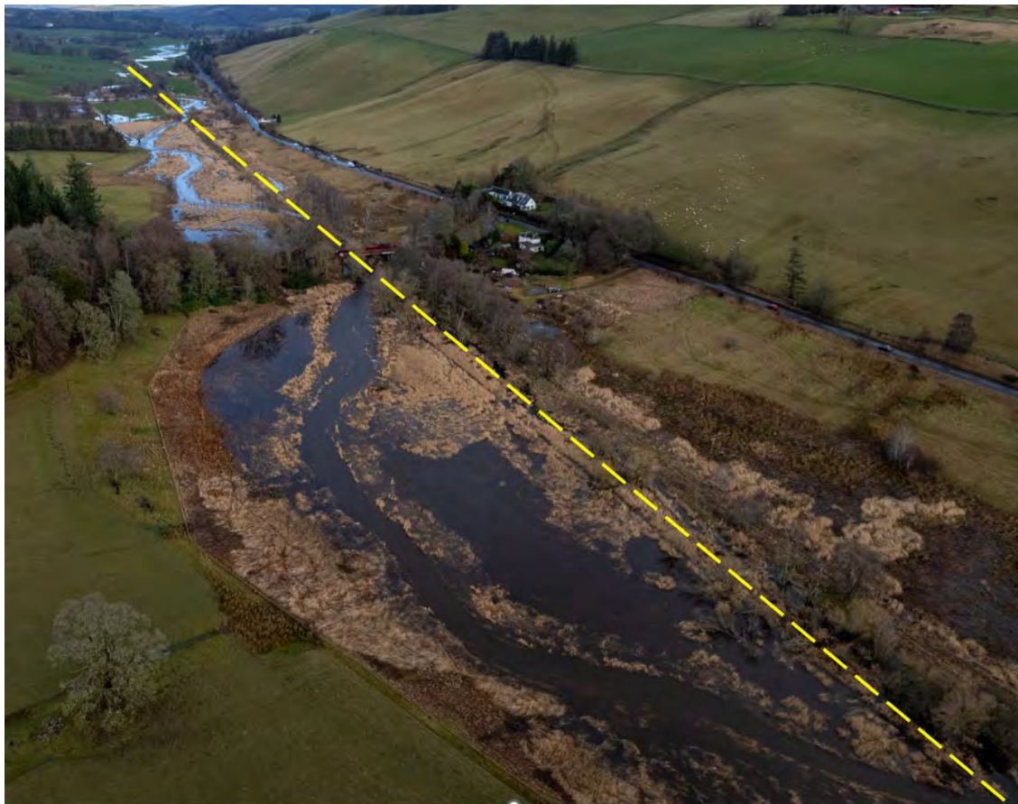
New meanders at upper Nether Kidston (foreground) and Cringletie upstream in flood conditions. The yellow line shows the line of the old straightened channel.
